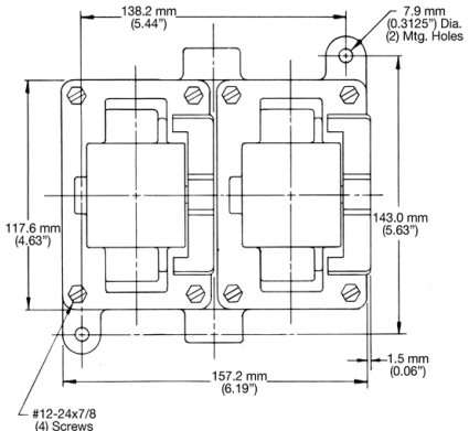
Front — 2-Gang
