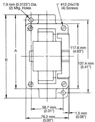
Front — 1-Gang
