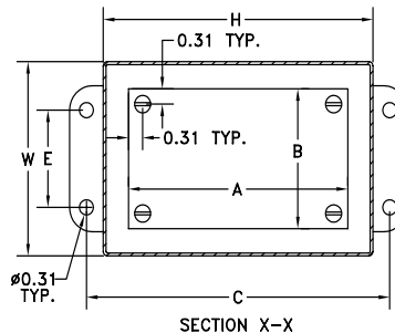
SECTION X-X
