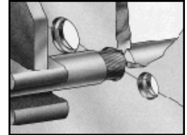
Die-type blades incorporate a counterbored hole sized to the insulation and an inner cutting hole sized to the conductor. This varies depending on insulation type and thickness.
