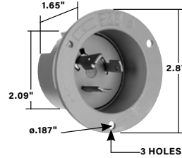
20A Flanged Inlet & Outlet
