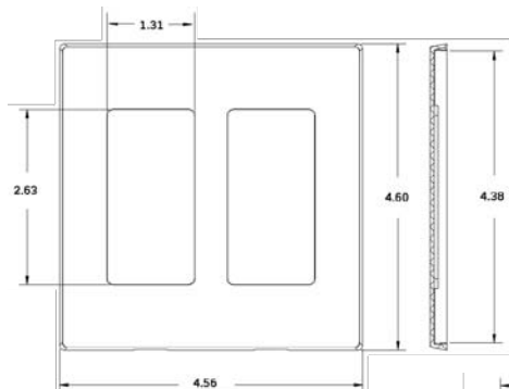
2-Gang Wallplate
