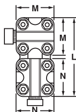
Elbow Cable to Cable or IPS to Cable or IPS to IPS
