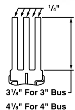
MULTI-TONGUE (ILLUSTRATION 3 BAR)
