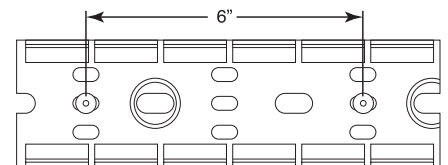
Minimum mounting rivet distance for ducts 1 1/2" to 2 1/4" wide.
