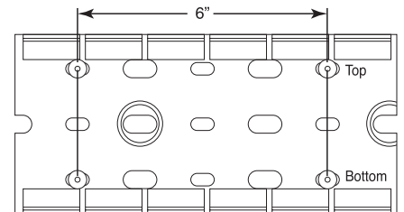
Minimum mounting rivet distance for ducts greater than 2 1/2" wide. Installed top and bottom.
